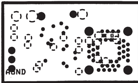
GROUND PLANE
